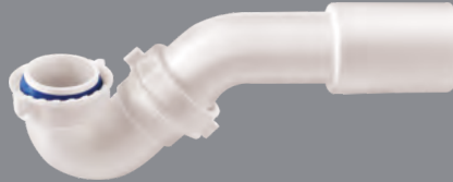
Ø 50 mm V-DİRSEK ÇIKIŞ Ø 40 mm - Ø 50 mm 3 DIMENSIONAL (FOR BATHTUBS AND SHOWER TRAYS)
